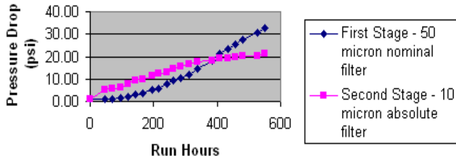
Fig. 4 Pressure Drop vs Run Hours for the Two Cartridge Filters in Series Process (4/4/2005 - 4/27/2005)
