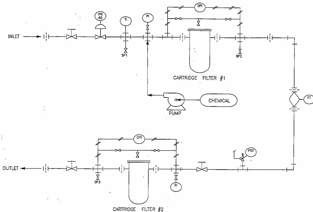
Fig. 1 Pilot Skid Layout
