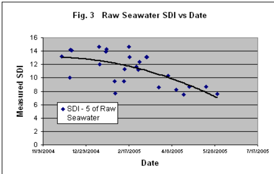
Fig. 3 Measured Feed Seawater SDI vs. Run Date
