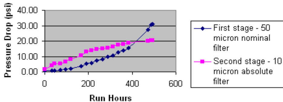
Fig. 5 Pressure Drop vs Run Hours for the Two Cartridge Filters in Series Process (4/27/05 - 5/18/05)
