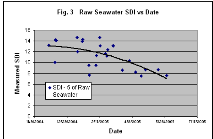
Fig. 3 Measured Feed Seawater SDI vs. Run Date
