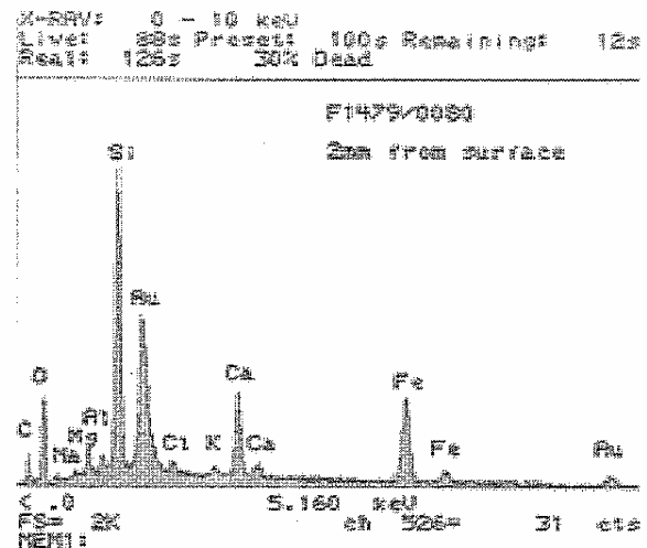
Fig. 10 Silicon, Calcium and Iron Measured by EDS
